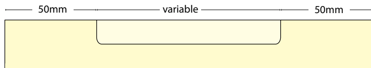
Scooped Rear Finger Pull FF08
