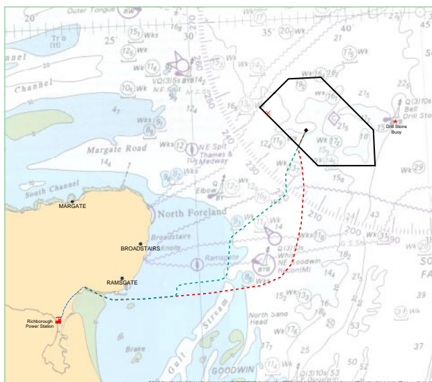
CABLE LAYING
